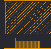
Hinged cover with floor covering recess and brush cord outlet
